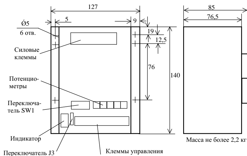
Рис.1. EI-MINI-LP2, LP4, LP7
